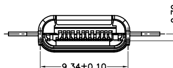
SECTION C-C SCALE 2:1
