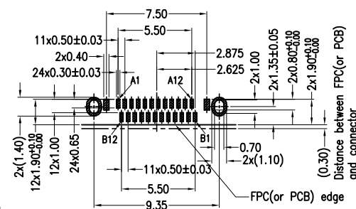
RECOMMENDED PCB LAYOUT DEFAULT TOLERANCE:±0.05
