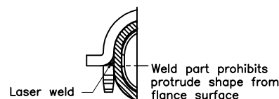
SECTION C-C SCALE 2:1
