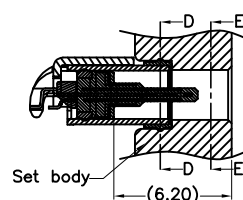
RECOMMENDED SET BODY SIDE HOLE SHAPE
