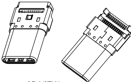
3D VIEW
