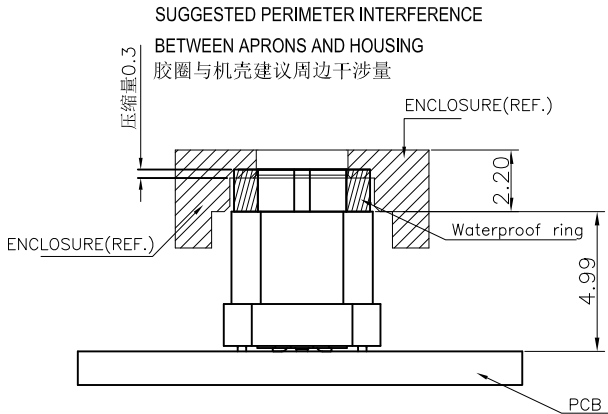
RECOMMENDED SCHEMATIC DRAWING OF CONNECTOR MATCH CHASSIS
