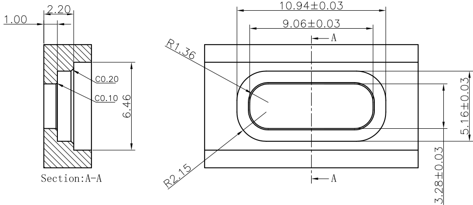
机壳开孔尺寸图 SIZE DRAWING OF OPENING HOLE OF HOUSING
