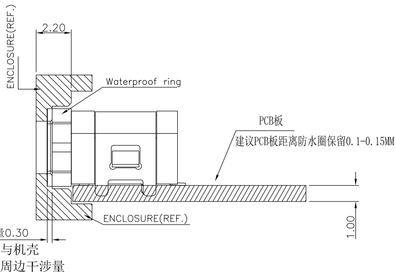
RECOMMENDED SCHEMATIC DRAWING OF CONNECTOR MATCH CHASSIS
